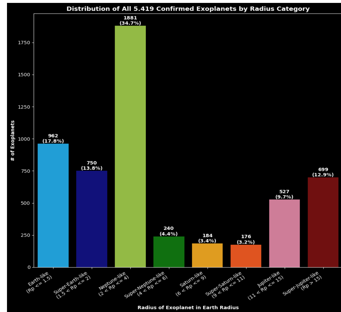
Figure 20: Bar Chart of Radius Characterization for all 5,419 Exoplanets which orbits a Main Sequence (V), Sub Giant (IV), Red Giant (III) Host Star.
