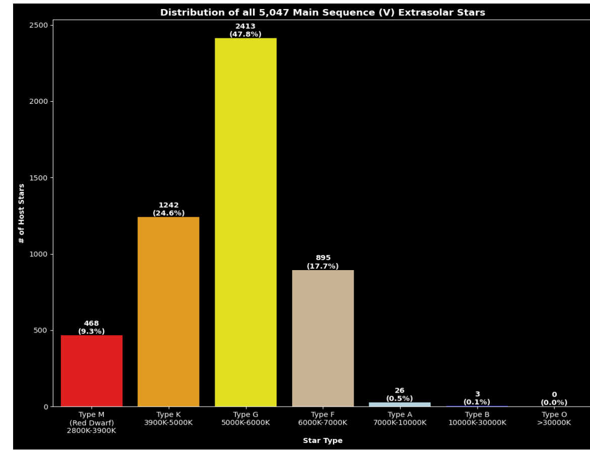
Figure 18: Bar Chart of the Distribution of all 5,047 Main Sequence Extrasolar Stars Characterized by spectral type
